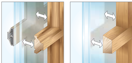
Ovolo (shown with permanent exterior grille)
